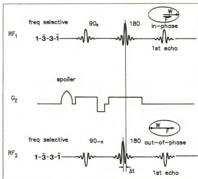
Fig. 1. —Diagram of hybrid pulse sequence used in this study. A frequency-selective pulse centered on fat resonance (in this case the 1331 pulse described by Hore [8]) is followed by chopper fat signal elimination. Two independent mechanisms of fat suppression applied together in one sequence substantially improve the effectiveness of fat/water signal separation.
