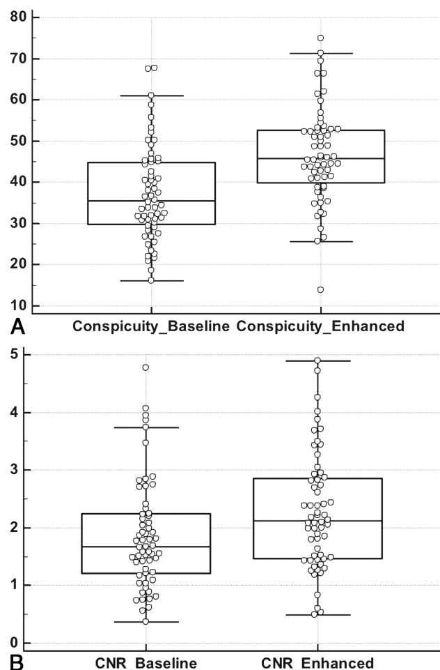
FIG 3. Boxplots showing the distribution of gray matter conspicuity (A) and CNR between gray and white matter (B) in 60 paired head CT images with normal findings before (baseline) and after (enhanced) processing with CIE. Both of these quantitative measures of gray-white differentiation demonstrated significant improvement following image processing ( P < .001 for conspicuity; P = .015 for CNR).
