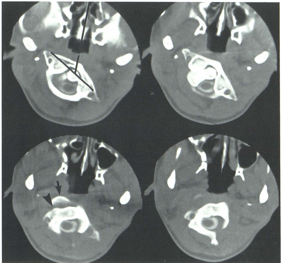
Fig. 1.—Case 5: 17-year-old girl with no history of trauma. Her head was fixed in rotation to the left and she had difficulty swallowing. Sequential CT scans from metrizamide myelogram show occipitatlantal dislocation and atlantoaxial rotary fixation. Septal axis forms acute angle with transverse axis of atlas. Right lateral mass of C1 (arrow) is displaced anterior to superior articular surface of C2 (arrowhead). Odontoid remains in normal relationship to anterior arch of atlas, suggesting that transverse ligament remains intact.
