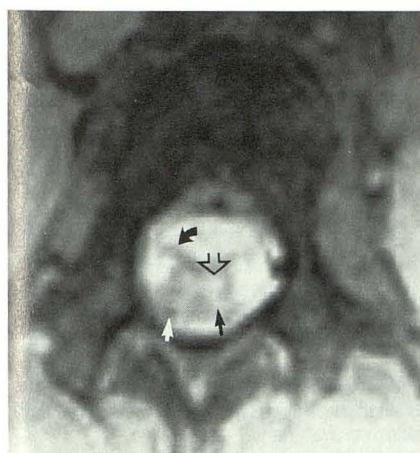
Fig. 8.—Demonstration of normal axial anatomy of lower thoracic spine by GRE. Note excellent definition of central gray matter including dorsal (solid straight black arrow) and ventral (open arrow) gray columns. Ventral roots are well visualized (curved arrow). Dorsal white matter (white arrow) can be seen easily.
