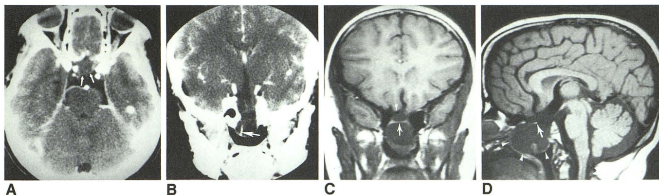
Fig. 1.—A, Axial enhanced CT shows a lesion of soft-tissue density within sella, slightly denser than CSF (arrows). B, Coronal enhanced CT image shows herniation of third ventricle inferiorly through sphenoid bone into epipharynx. Enhancement of infundibular stalk can be seen inferiorly in encephalocele (white arrow). C, Coronal MR (SE 800/20) shows optic chiasm (arrow) displaced inferiorly within encephalocele. Lateral to chiasm and encephalocele wall, internal carotid arteries and aerated sphenoid bone can be seen as regions of signal void. A1 segment of right anterior cerebral artery lies just above encephalocele (arrowhead). D, Sagittal MR (SE 800/20) shows inferior extension of third ventricle into encephalocele. Ptotic optic chiasm (arrow) is somewhat thin. Encephalocele bulges into epipharynx (arrowheads).
