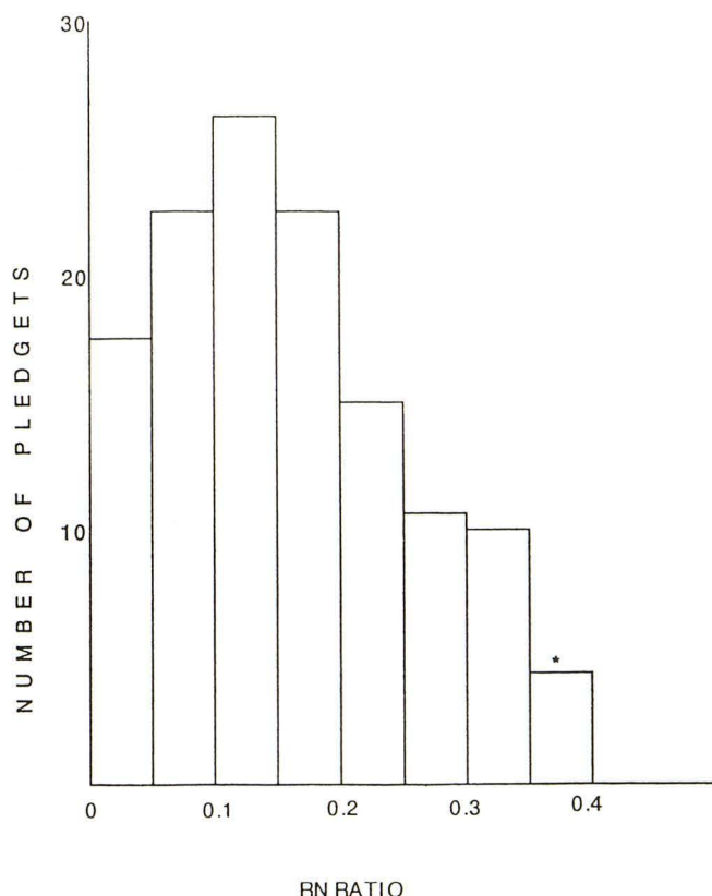
Fig. 3.—Radionuclide (RN) counts in normal subjects.
