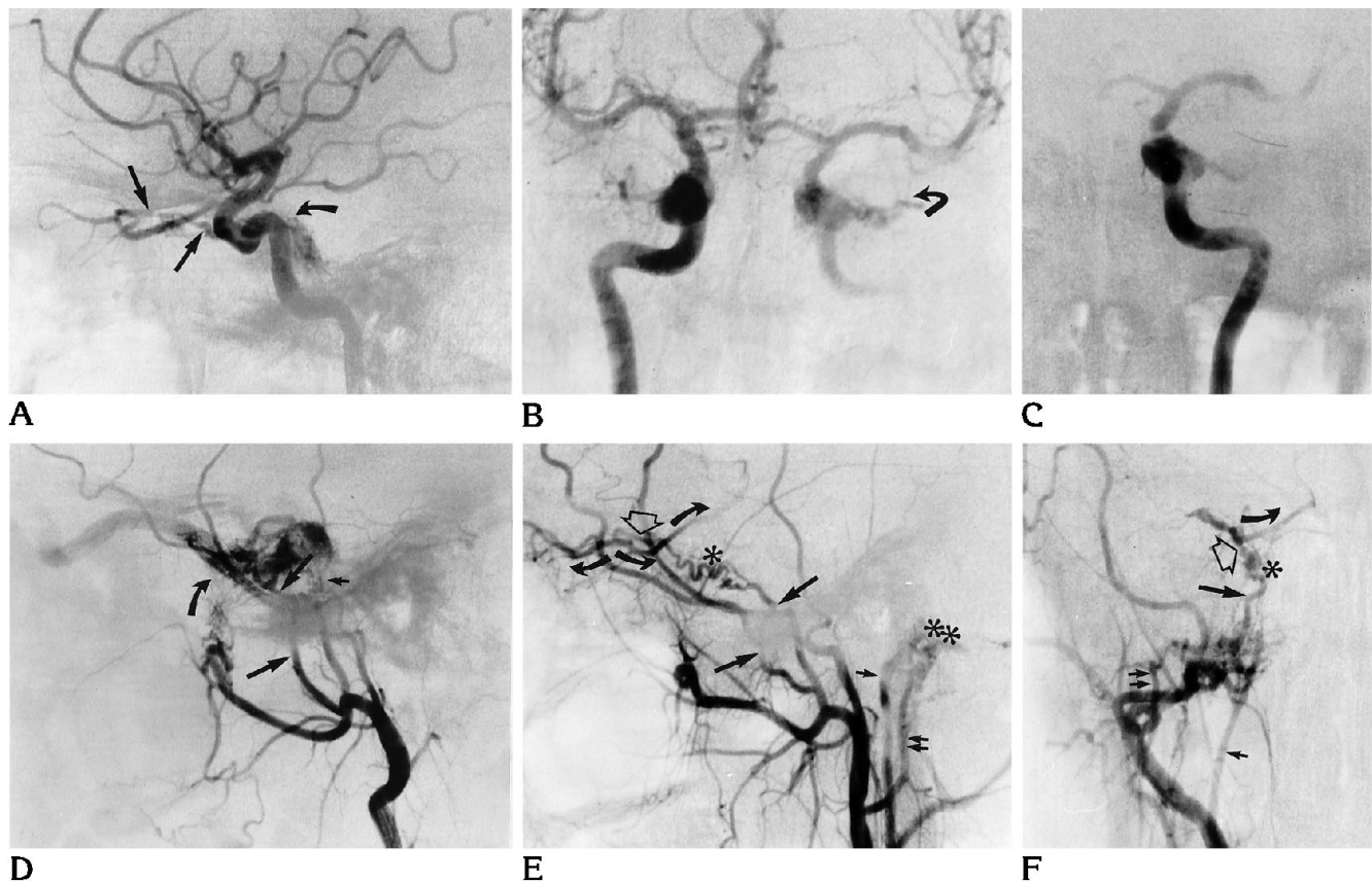
Fig 1. A, Left internal carotid angiogram demonstrates a carotid-cavernous fistula with main supply by the deep recurrent ophthalmic artery (arrows). There also is filling of the cavernous sinus through cavernous branches from the C-5 segment (curved arrow).
