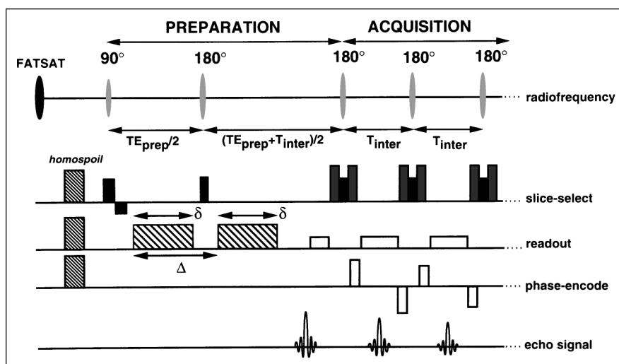
FIG 1. Schematic representation of the basic diffusion-weighted HASTE sequence. Sensitization to diffusion is achieved by a preparation period (spin-echo scheme with diffusion gradients, denoted by hatched patterns and TE_{prep}/2 ). The transverse magnetization at the end of the preparation period is imaged by a HASTE sequence. Gradient pulses ( positive and negative black blocks ) indicate the section (slice) selection gradients and section (slice) select rephasing gradients. Gradient pulses ( gray patterns ) correspond to balanced pairs of crusher gradients in section (slice) direction around the refocusing pulses.
