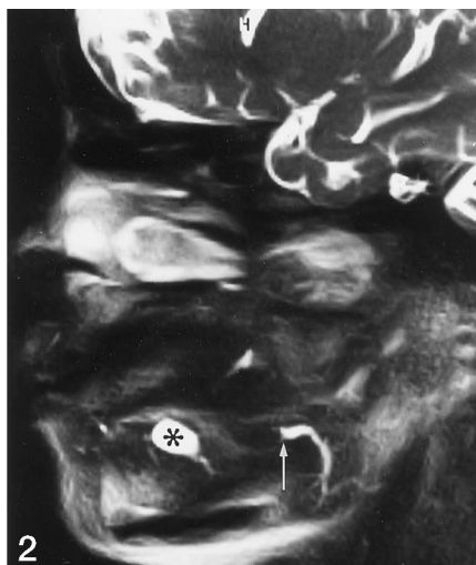
FIG 2. 58-year-old woman with inflammatory stenosis of the right submandibular gland duct who had been treated previously for a right submandibular calculus. An oblique sagittal image of the right submandibular gland duct shows obstruction (arrow) and dilatation in the posterior part of the duct. The point of obstruction corresponded to the findings of X-ray sialography. Ranula in the right sublingual gland (asterisk) is also seen.
