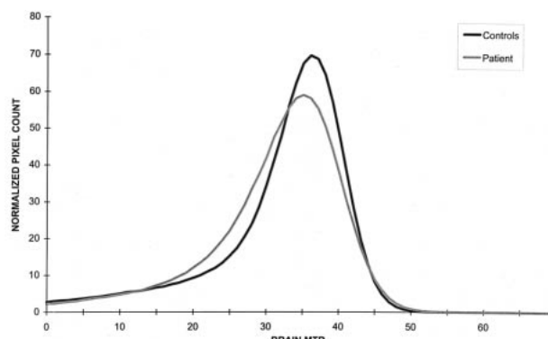
FIG 2. MT histograms of a patient with CDMS, obtained before the onset of clinical symptoms ( gray line ), and MT histograms of 10 healthy control volunteers ( black line ).
