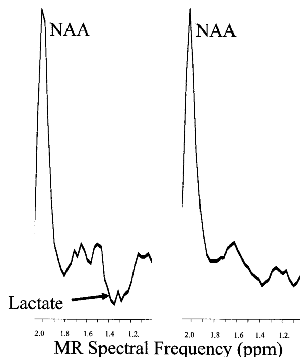
FIG 3. Baseline-corrected proton spectra from a dyslexic participant in the left frontal region of the brain shows significant lactate activation during the phonologic task. The inverted lactate proton doublet can be observed at 1.3 ppm during the phonologic task (left) but not during passive listening (right). The other resonance that can be observed in the spectra is NAA.
