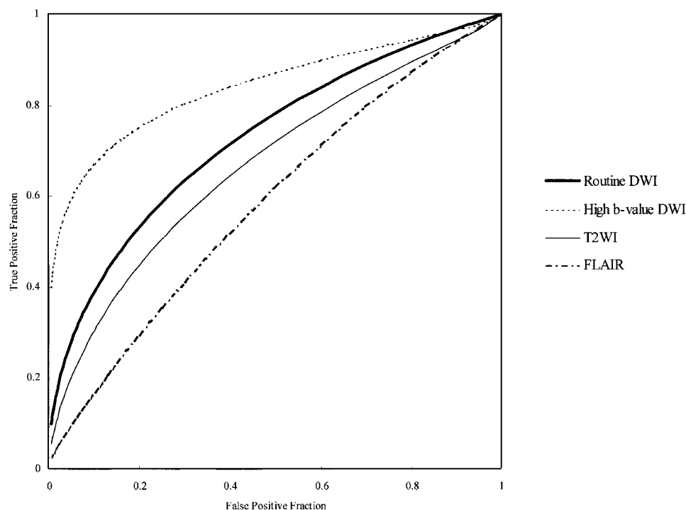
FIG 3. The ROC curves of each MR image achieved by the three observers. The high- b -value DWI holds the largest area under the curve ( A_z ). The A_z of the routine DWI ( b = 1000 s/mm 2 ), T2WI, and FLAIR imaging follow in descending order.
