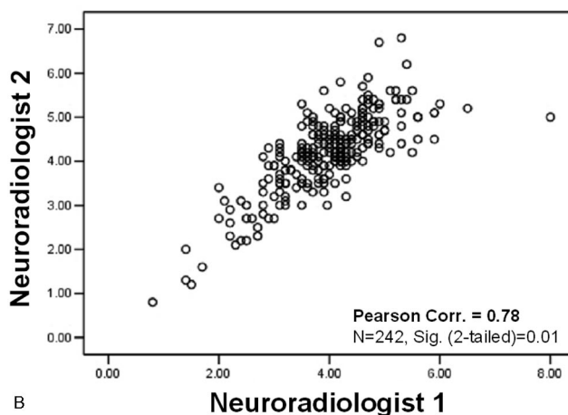
Fig 4. Correlation scatter plots. Interobserver agreement between reader measurements. A, Maximum stenosis (mm). B, Distal ICA (mm). C, Derived NASCET-style percent stenosis. (Correlations: 2-tailed significance = 0.01. n values reflect exclusion of pairwise missing data; excludes "near-occlusion" cases).
