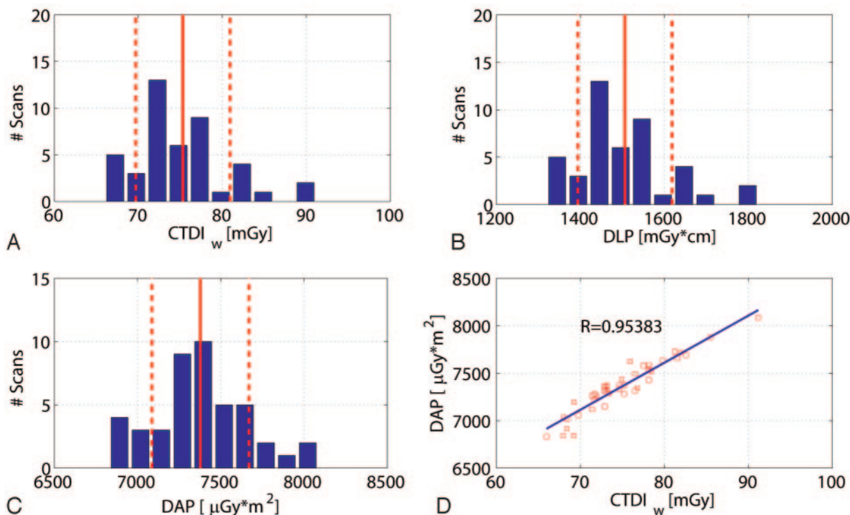
Fig 5. Dose values for 45 patient scans with use of the high-quality protocol. A, B, and C show the histogram of patient scans with respect to the CTDI, DLP, and DAP. The distributions are similar for the 3 dose measurement techniques. The DAP measured on-line shows a good linear correlation to the estimated CTDI_w value (D). Note: The red lines and red dotted lines indicate the mean value and SD.
