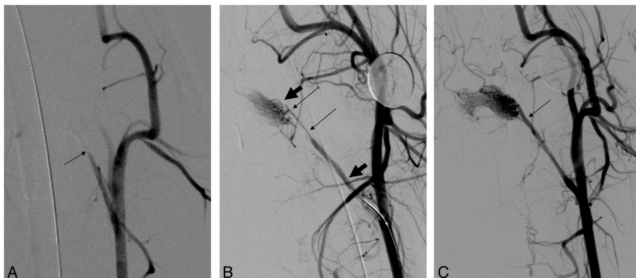
Fig 2. A , Anteroposterior angiogram of the left common carotid artery in swine. Occlusion of the APA is seen (arrow). B , Right anterior oblique angiogram of the left common carotid artery with the device deployed shows immediate flow restoration. The thin arrows indicate the proximal and distal aspects of the clot, while the thick arrows point to the proximal and distal ends of the device. C , Right anterior oblique angiogram of the left common carotid artery postretrieval of the clot shows complete restoration of flow. Arrow shows the original site of occlusion.
