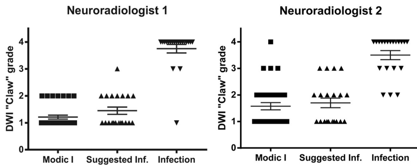
FIG 4. A, Modic type 1 = 1.21 \pm 0.07 ; suggested infection = 1.45 \pm 0.13 ; proved infection = 3.75 \pm 0.16 . B, Modic type 1 = 1.58 \pm 0.14 ; suggested infection = 1.70 \pm 0.18 ; proved infection = 3.50 \pm 0.17 .
