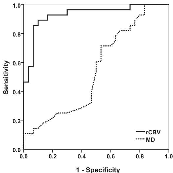
FIG 2. Receiver operating characteristic curves of rCBV_{max} (solid line) by using a rCBV_{max} cutoff value of 5.79. The area under the curve was 0.93. The receiver operating curve of MD_{min} (dotted line) by using a cutoff value of 8.35 \times 10^{-4} \text{ mm}^2/\text{s} demonstrated only a modest area under the curve of 0.55.
