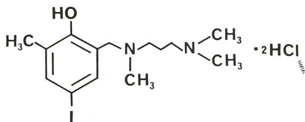
Fig. 1.—N,N,N'-trimethyl-N'-(2-hydroxyl-3-methyl-5-iodobenzyl)-1,3-propanediamine · HCl (HIPDm).
