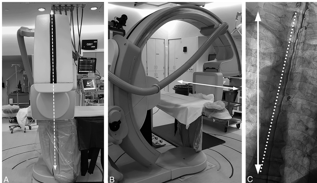
FIG 4. Defining the true horizontal axis and spine tilt on DSM. By placing the C-arm in a vertical position with respect to the floor (A, dotted arrows) while maintaining the long axis of the image intensifier orthogonal to the C-arm (B, solid arrow), the long axis of the image intensifier and the long axis of the image are aligned horizontally, parallel to the floor (B and C, solid arrow). The angle between this line and the line connecting the spinous processes (C, dotted line) defines the spine tilt with respect to the floor.
