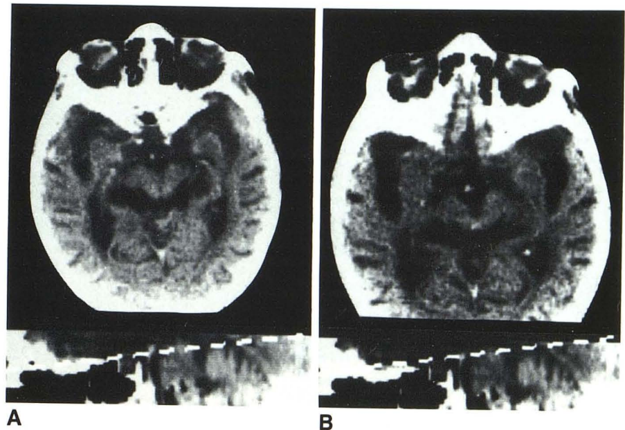
Fig. 1.—Case 5. Reformatted midbrain CT scans on GE scanner. A , Atrophy, dilated aqueduct, and enlarged cisterns. B , Low-density midline abnormality. Reformatted images were nearly identical to those obtained with Philips scanner (cf. figs. 6A and 6B).
