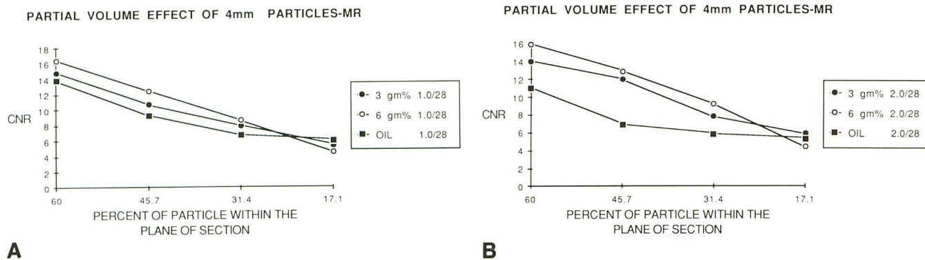
Fig. 7.—Experiment 2. Contrast-detail curves showing the effect of partial volume on 4-mm particles.
