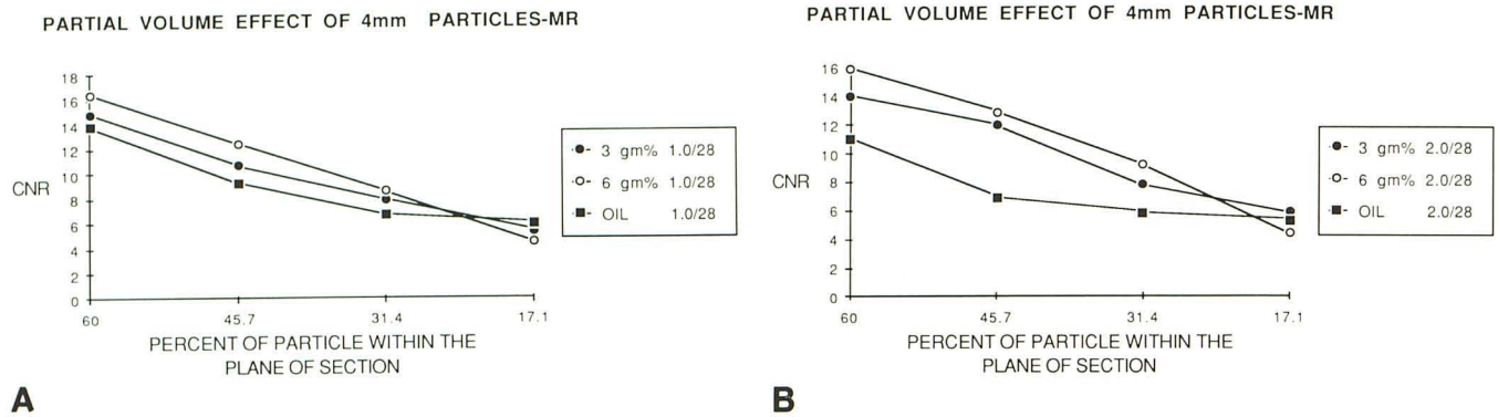
Fig. 7.—Experiment 2. Contrast-detail curves showing the effect of partial volume on 4-mm particles.
