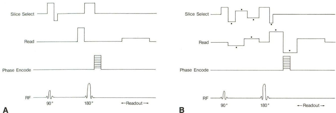
Fig. 5.—A, Gradient waveforms used in a conventional spin-echo pulse sequence.
