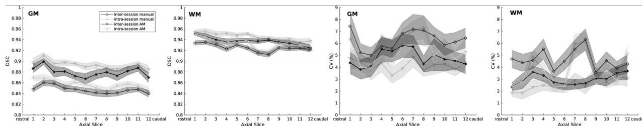
FIG 4. Comparison between the reproducibility of manual and automatic measurements (AM) of spinal cord gray matter and white matter per axial slice. Intrasection and inter-session reproducibility is assessed in terms of Dice coefficients (graphics on the left) and coefficients of variation (graphics on the right). Manual and automatic inter-session reproducibility is shown in dark gray, whereas manual and automatic intrasection reproducibility is shown in light gray. Error bars display mean values \pm 0.2 SDs.
