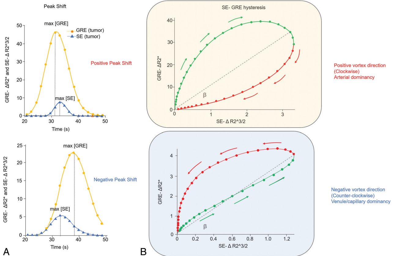
FIG 2. Peak shift and hysteresis plot. A, Peak shift: the time curves of GRE-based \Delta R2^* and SE-based \Delta R2^{3/2} were fitted to a \gamma -variate function. A positive peak shift indicates a GRE peak preceding the SE peak, while a negative peak shift indicates the SE peak preceding the GRE peak. B, Hysteresis plot: the fitted curves are plotted with \Delta R2^{3/2} (SE-based) along the x-axis and \Delta R2^* (GRE-based) along the y-axis. The clockwise rotation indicates that GRE-based changes precede SE-based changes, corresponding to the positive peak shift with arterial dominance. The counter-clockwise rotation indicates that SE-based change precedes GRE-based changes, corresponding to the negative peak shift with venous dominance. Max indicates maximum.
