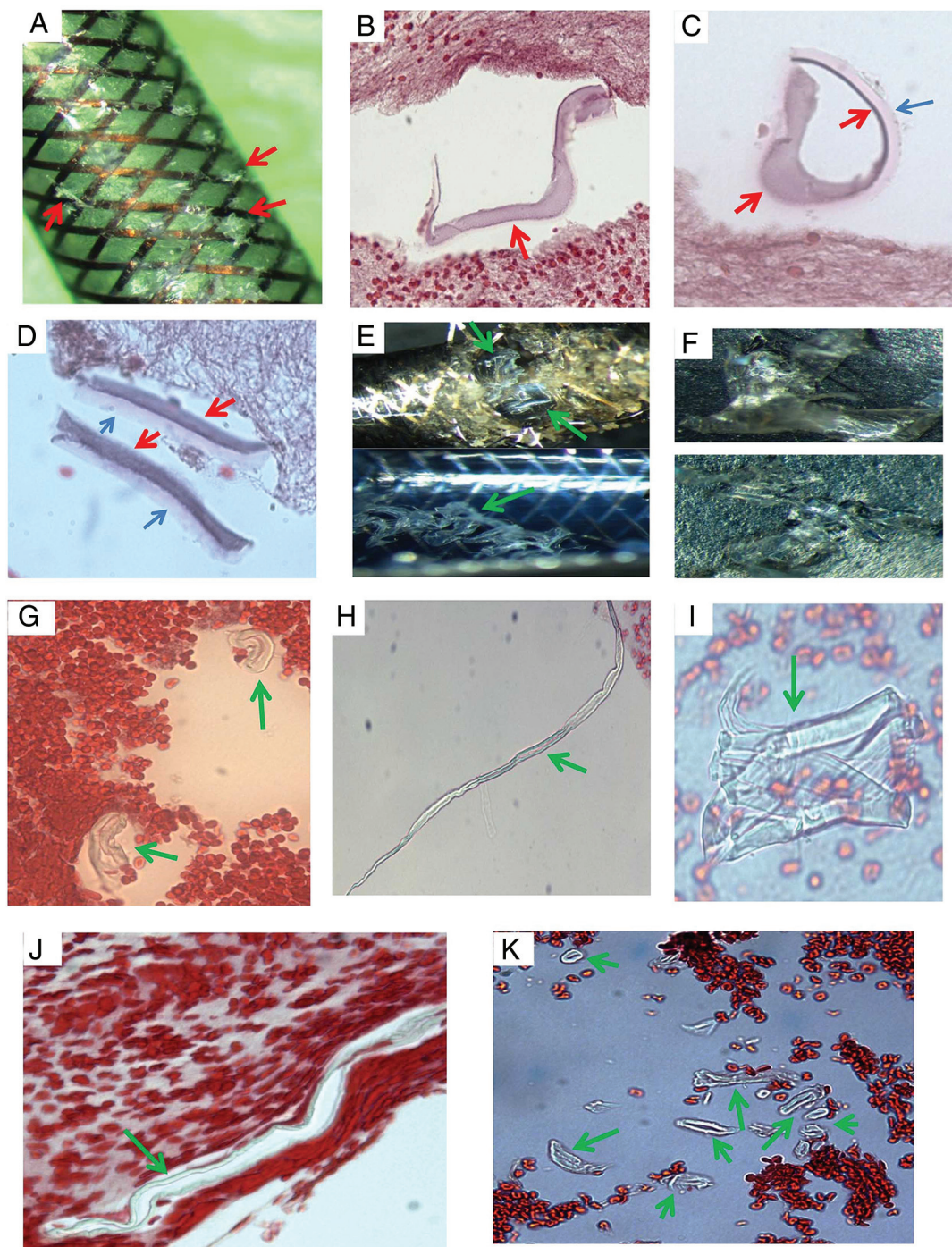
FIG 2. Histologic appearance of scratched surface and inner layer of MT catheter. A , Macrophotograph of the Sofia catheter, showing the scratched surface pieces ( red arrows ). B–D , Microphotograph of scratched pieces from image A associated with clot analog tissue, showing the surface-coating material, which appears to be varied in shape and texture following tissue processing ( red arrows ), and which is similar to the material seen in the cross-section experiment ( Fig 1 ). The layer immediately underneath the surface-coating material is also present ( blue arrow ), which appears to be a different shape, light pink/red, and has a homogeneous texture. It is similar to the material seen in the cross-section ( Fig 1 , blue arrow ), and type IV foreign material ( Fig 8 ) found in the patient clot tissue as well. E , Macrophotograph of Sofia and Fubuki catheters, showing the scratched liner layer material in situ ( green arrows ; upper—Sofia; lower—Fubuki). F , Macrophotograph of the manually torn off liner material pieces from image E , showing the similar gross appearance to that of the PTFE material ( Fig 4 ). These pieces were crushed into small pieces for further routine, histologic processing, similar to the surface scratched material mentioned in Fig 1 . G–I , Microphotograph of torn off liner pieces from F (upper), showing the material that appears to be varied in shape, color, and texture because of processing. These could be tube-like, long stripe, or an irregular solid mass, with refraction and light green outline. Those features are the same as what is seen from the PTFE material ( Fig 4 ), and the type I material found in the patient clot ( Fig 5 ). J and K , Representative microphotograph of scratched, torn off liner pieces from F (lower), showing the material that appears to be long, or short, or small tubular in shape, and light green, as shown with the PTFE material ( Fig 4 ) and type I foreign material found in the patient clot tissue ( Fig 5 ).
