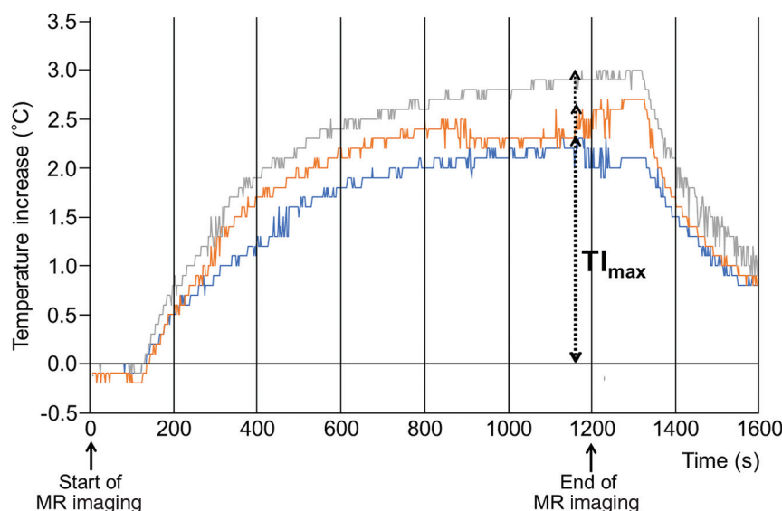
FIG 3. Chronological changes in the TI at 3 locations for the long straight clip. TI (degrees Celsius) indicates the difference between temperatures before MR imaging and during or after MR scanning (latter-former). Blue, orange, and gray lines denote the TI at tip of the clip head, tip of the clip blade, and 5 mm from the tip of the clip blade, respectively. TI_{max} indicates maximum TI at each location.
