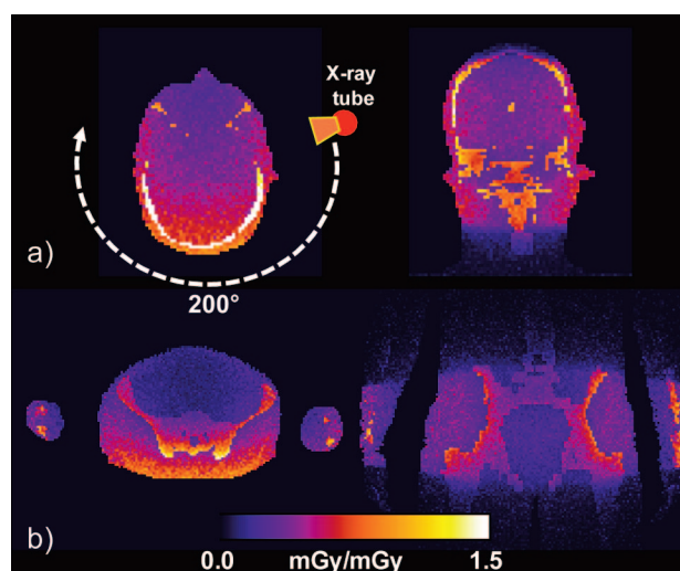
Fig 8. Example of 3D dose distributions calculated by Monte Carlo simulations for 2 phantom planes (axial and coronal) with use of an anthropomorphic phantom for a 200° C-arm FPCT scan in relative units representing head and pelvis scans. The axial section nicely demonstrates the inhomogeneity of the dose distribution for a partial scan.
