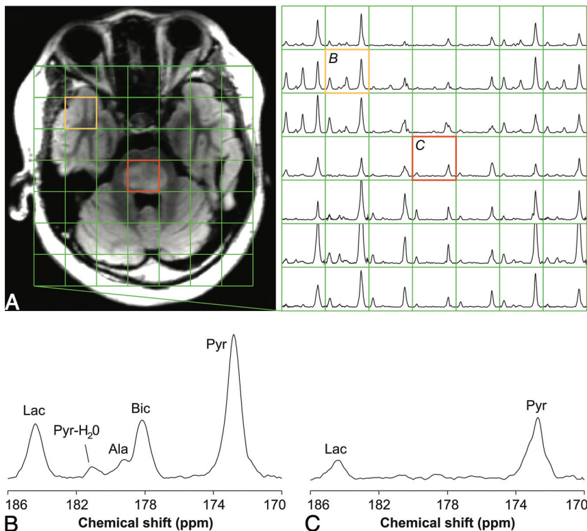
FIG 2. HP- 13 C spectroscopy of DIPG. HP- 13 C EPI of a 12-year-old male participant (P-02) with DIPG following injection of HP [1- 13 C]pyruvate. Temporally summed 13 C spectra are shown together with their spatial correspondence to a 1 H FLAIR image from the center of the 2-cm-thick 13 C volume (A). Spectra from normal-appearing tissue (B) and the lesion (C) illustrate individual HP metabolite resonances. The [ 13 C]bicarbonate resonance is aliased from 160.8 ppm. Pyr indicates [1- 13 C]pyruvate; Pyr-H 2 O, [1- 13 C]pyruvate-hydrate; Lac, [1- 13 C]lactate; Bic, [ 13 C]bicarbonate; Ala, [1- 13 C]alanine exclusively from outside the brain.
