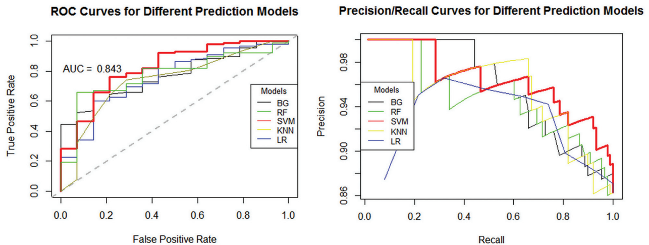
FIG 1. Performance of different machine learning models on an independent, external validation data set: A, ROC curves. B, Precision/recall curves. The best performance is achieved by the SVM model (red curves). BG indicates bagging or bootstrap aggregating; RF, random forest; SVM, support vector machine; KNN, K-nearest neighbor; LR, logistic regression.
